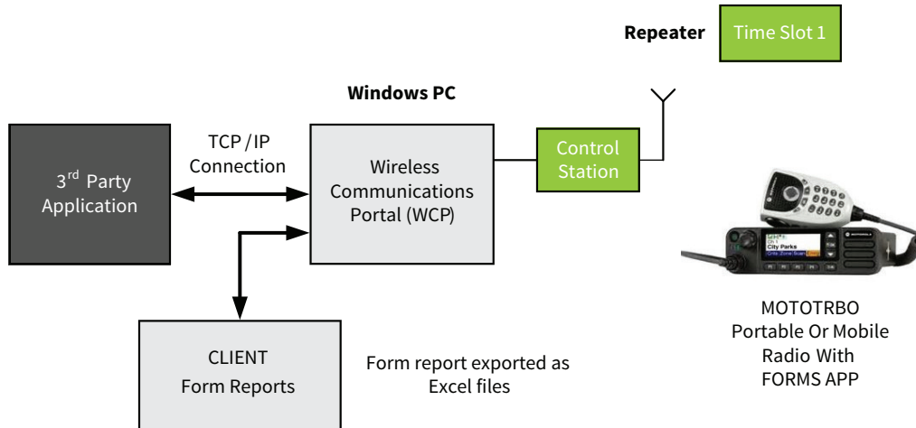
Figure 1: FORMS APP - Typical System Configuration
